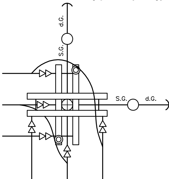
PRIMARY, TWO STUB GUYS, FOR LARGE LARGE ANGLES & HIGHER TENSIONS.
